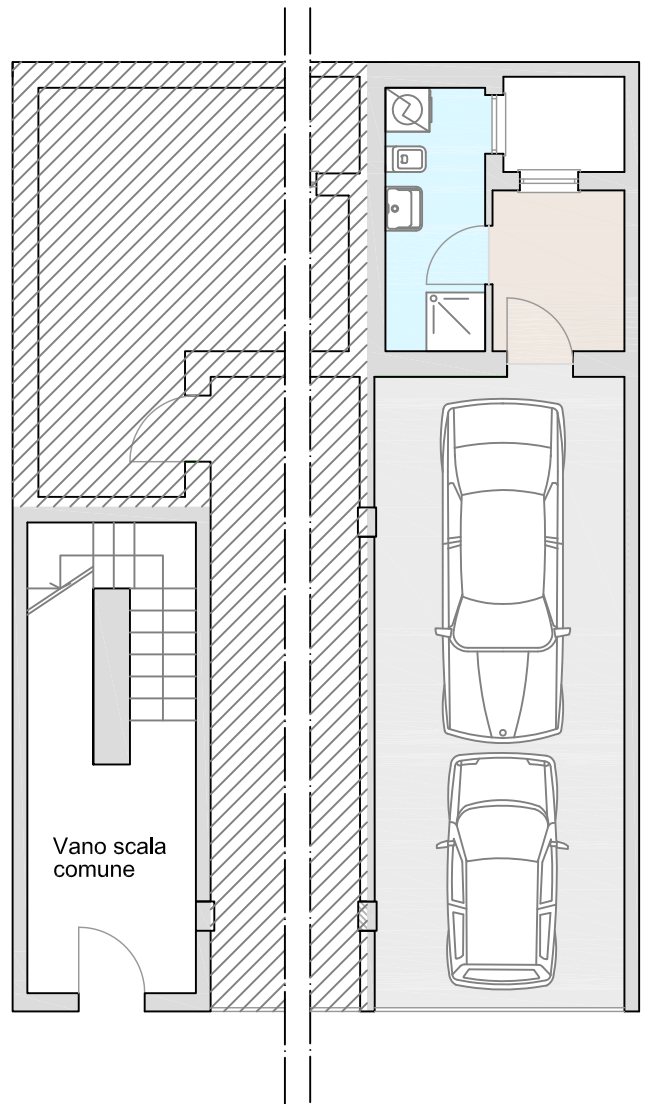
Piano Interrato
