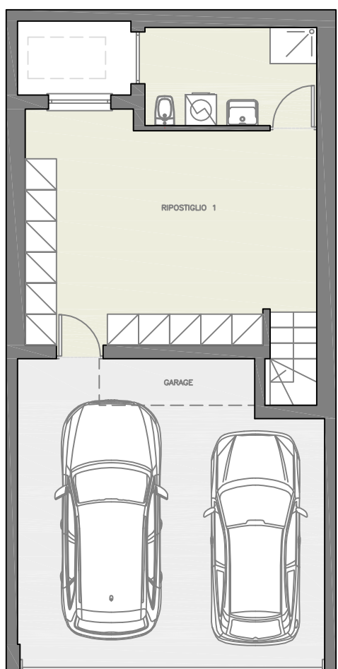
PIANO INTERRATO
